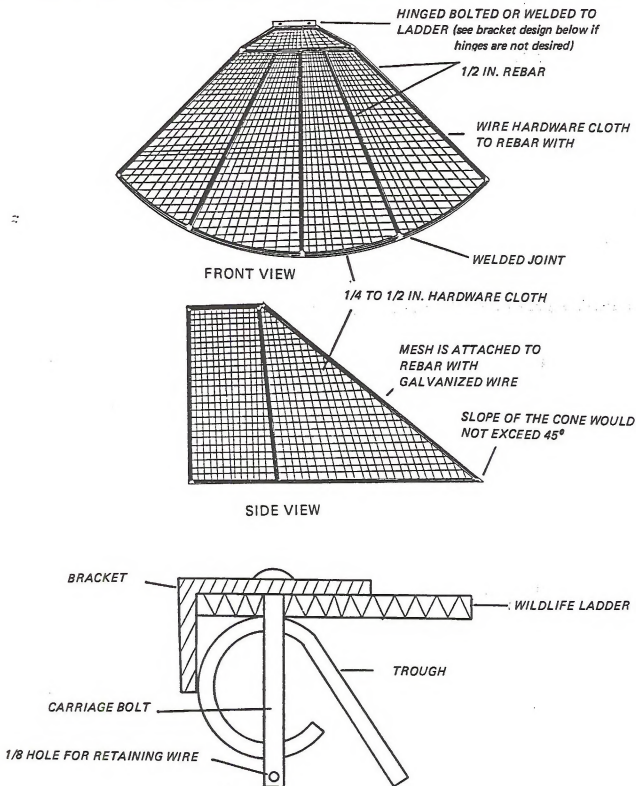
ILLUSTRATION 9: Cone shaped wildlife ladders are recommended for circular troughs.
